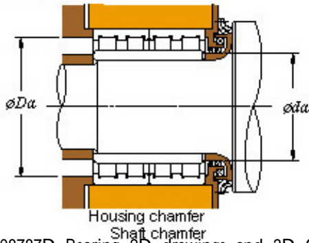
152FC108787D Bearing 2D drawings and 3D CAD models
